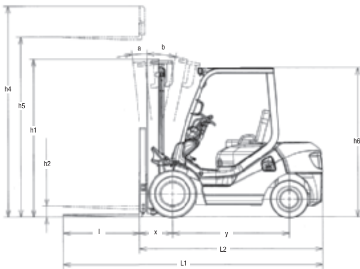
Dimensions of the FG25T-16
