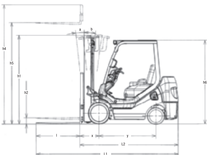
Dimensions of the FG25ST-16
